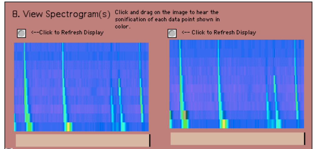
SWAVES type-3 bursts, Nov. 22 + 5hrs
