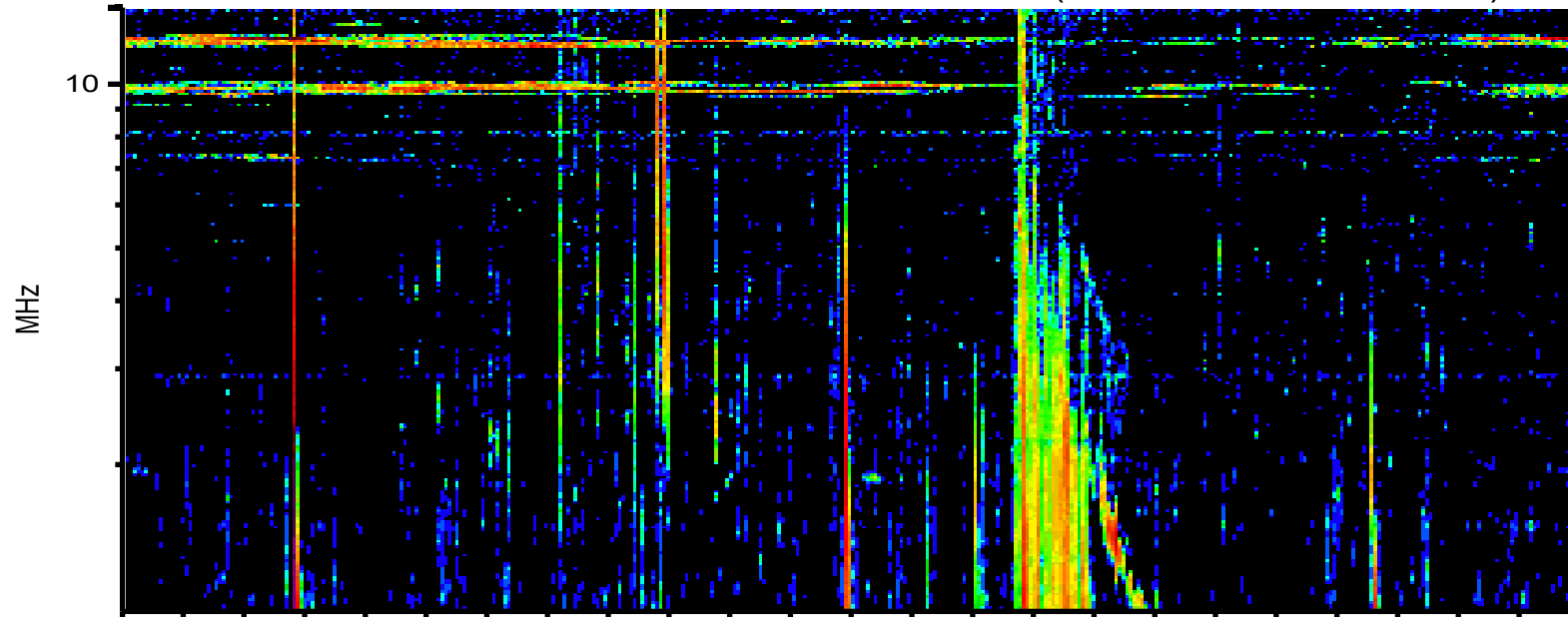
Wind Waves RAD2 receiver: 2005/8/23 (1 min X 50 kHz resolution)
